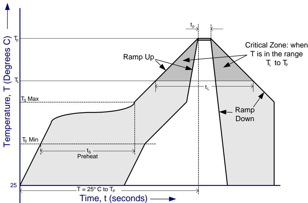
Figure 9.3 FT245R Solder Reflow Profile
