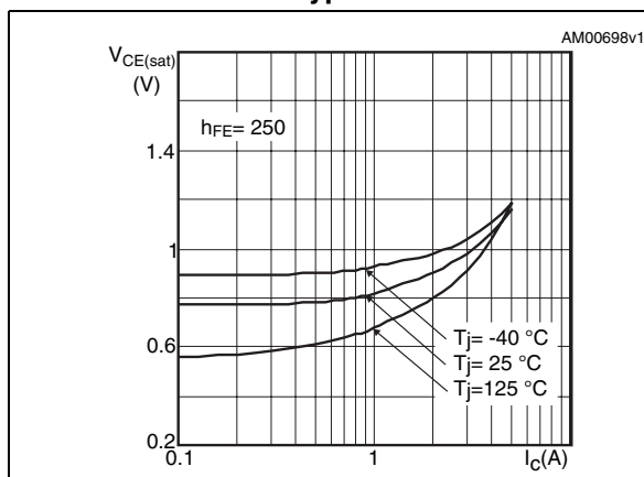
Figure 6. Collector-emitter saturation voltage for NPN type
