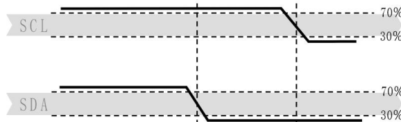
Figure 10. Start transmission status (S)
